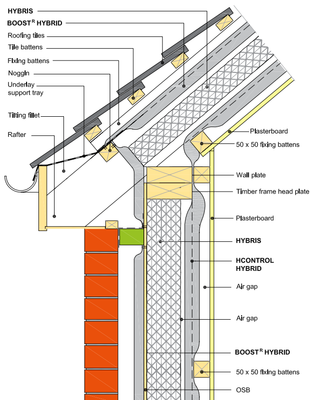
HY11 - EAVES DETAILS
